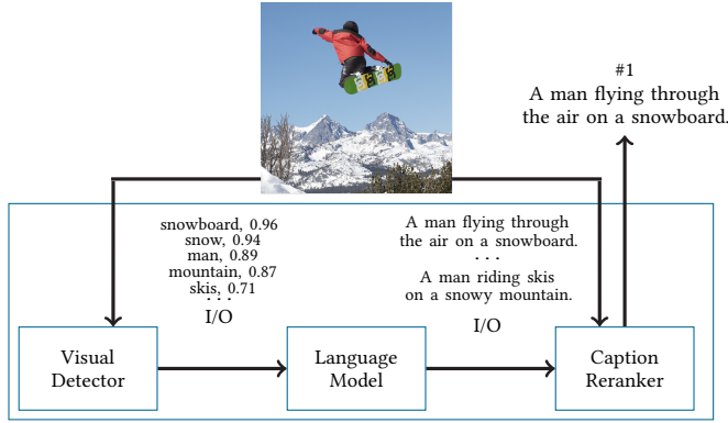
Figure 2: The image captioning system.
